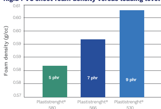
Rigid PVC sheet foam density versus loading level
